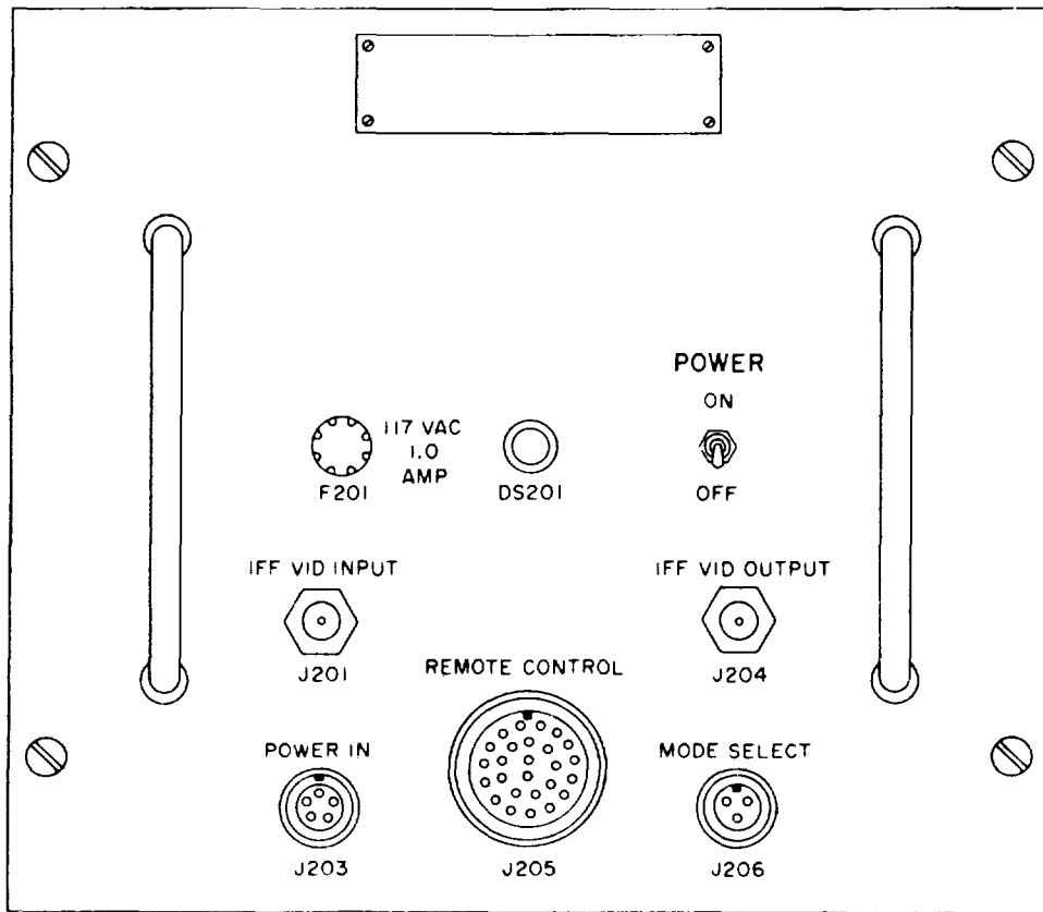
Figure 3-6. Decoder, Video KY-593/TPX-44, controls and indicators.
