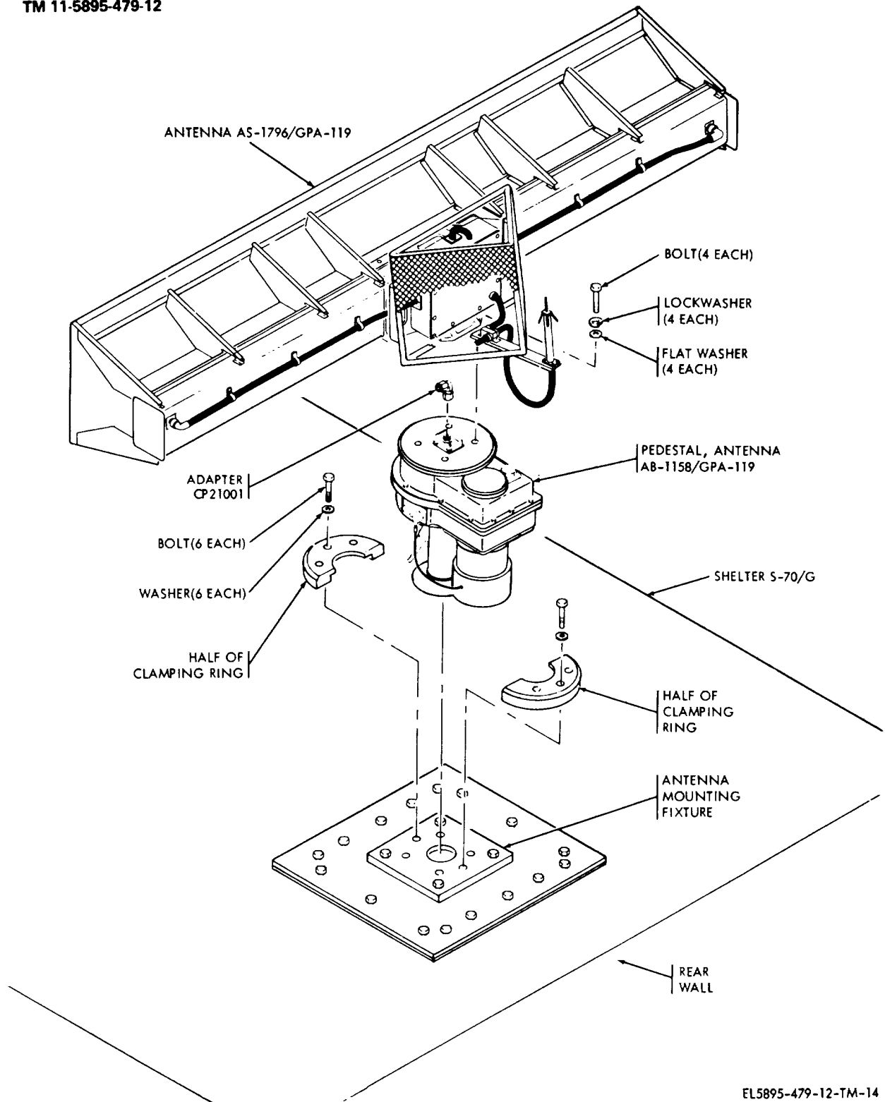
Figure 2-11. Antenna Group AN/GPA-119, installation diagram.
