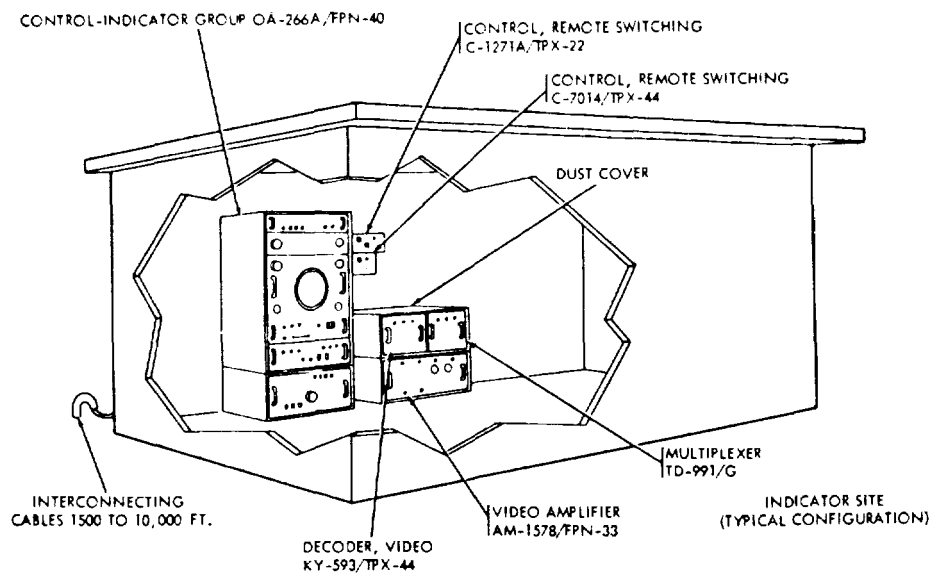
Figure 2-8. Interrogator Set AN/TPX-41, siting diagram.
