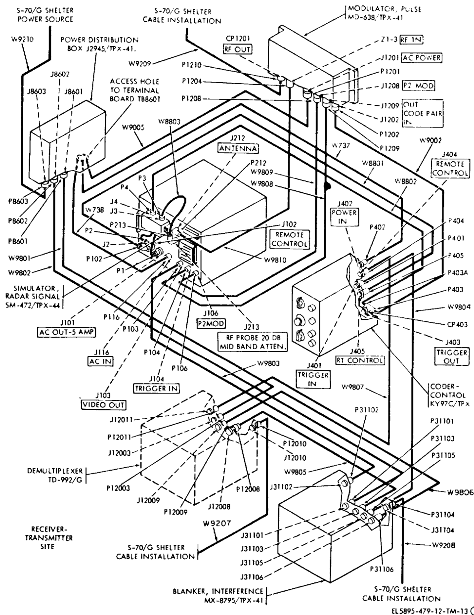
Figure 2-10(1). Interrogator Group OA-7487/TPX-41, cabling diagram (sheet 1 of 2)
