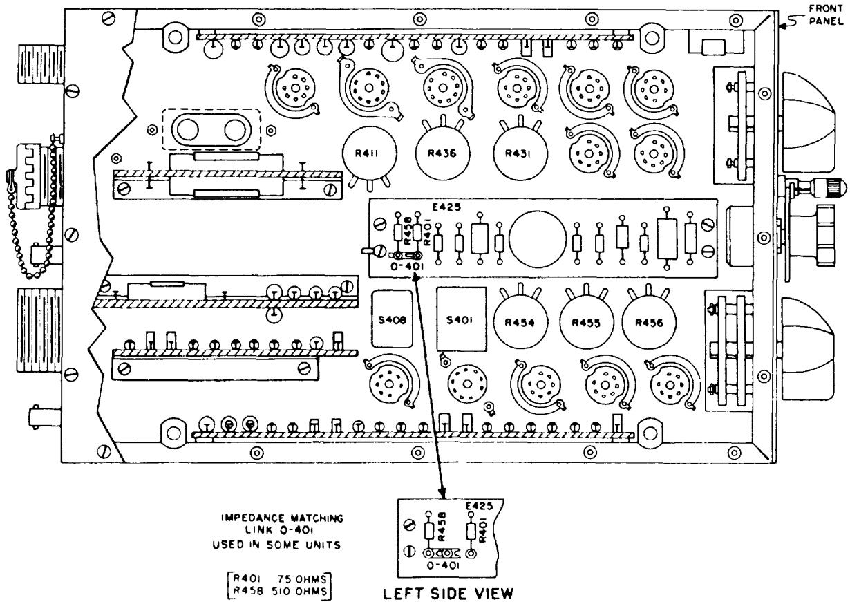
Figure 2-16. Coder Control KY-97C/TPX, initial adjustments.
