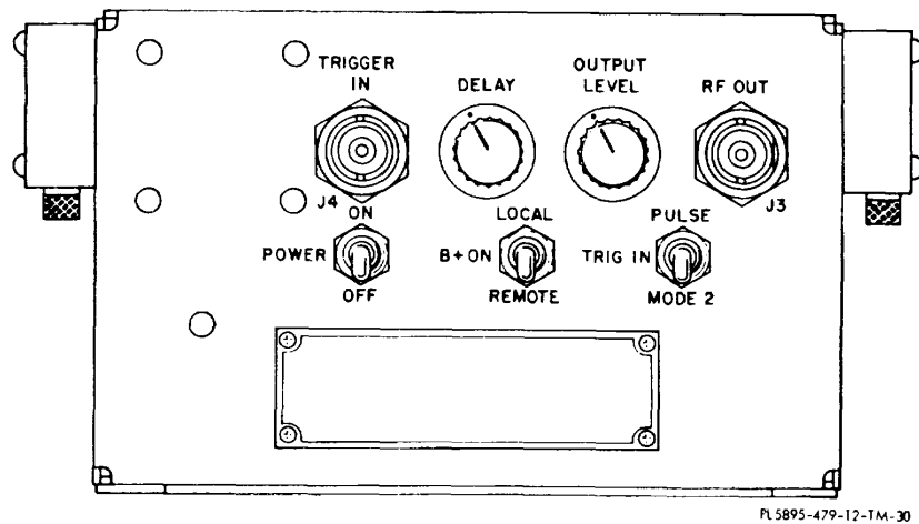
Figure 3-9. Simulator, Radar Signal SM-472/TPX-44, controls and indicators.
