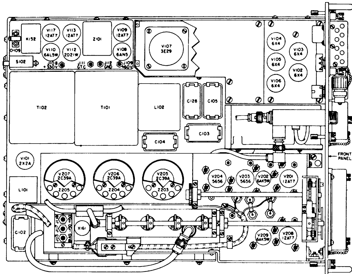
TOP VIEW
